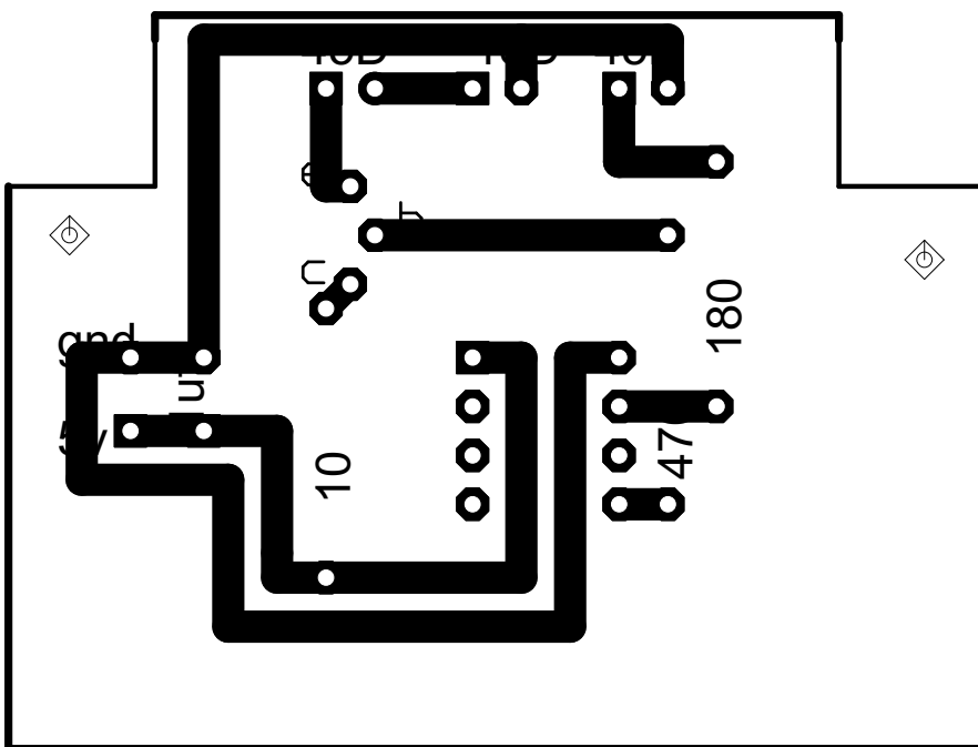
This version uses an NPN transistor for two high power LEDs
